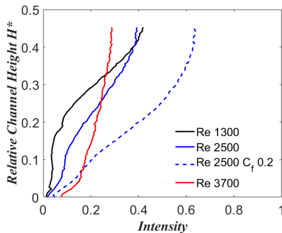
Figure 5: Fibre intensity over the channel height normalized with the channel height H .
