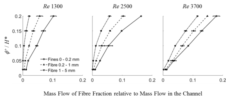
Figure 8: Fines and fibre removal characteristic for different Reynolds numbers Re .
