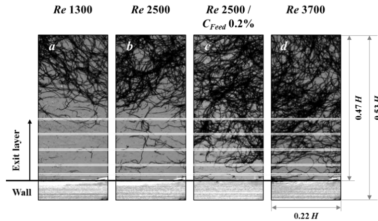
Figure 3: Snapshot of the fibre suspension flow just before the side channel exit for Reynolds numbers Re of 1300 (a), 2500 (b), 2500, and 3700 (d). Panel c shows the case of 0.2% fibre concentration at Re 2500, while all other cases are at a concentration of 0.1%. The black line indicates the channel wall. White lines indicate the averaged exit layer position for \phi^+ of 0.02, 0.05, 0.10, 0.15, and 0.20.
