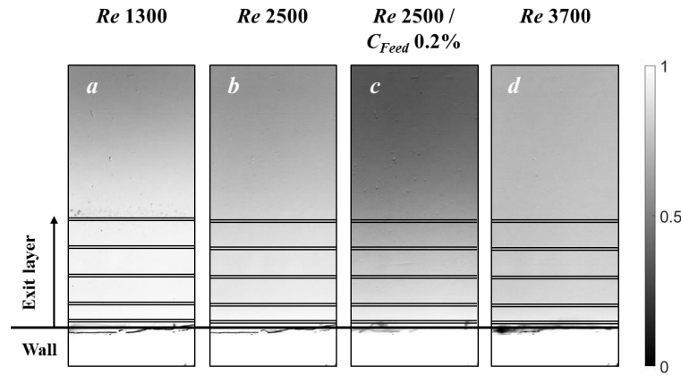
Figure 4: Time-averaged grey scale images associated with the snapshots presented in Figure 3. The wall is indicated by a solid line, while the height of the exit layer is indicated by a black double line. The colour bar states the dimensionless voidage: 1 solid, 0 no solid.
