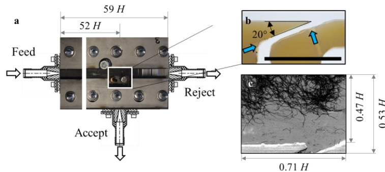
Figure 1: Hydrodynamic fractionation device (a) with magnification on the backwards facing separation channel (b). Purge water channels are indicated in with blue arrows. (c) is a snapshot of the suspension that has been recorded using a high-speed camera.
