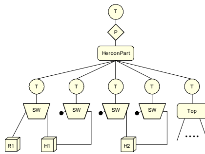
Fig 15: Scene graph for archaeology
