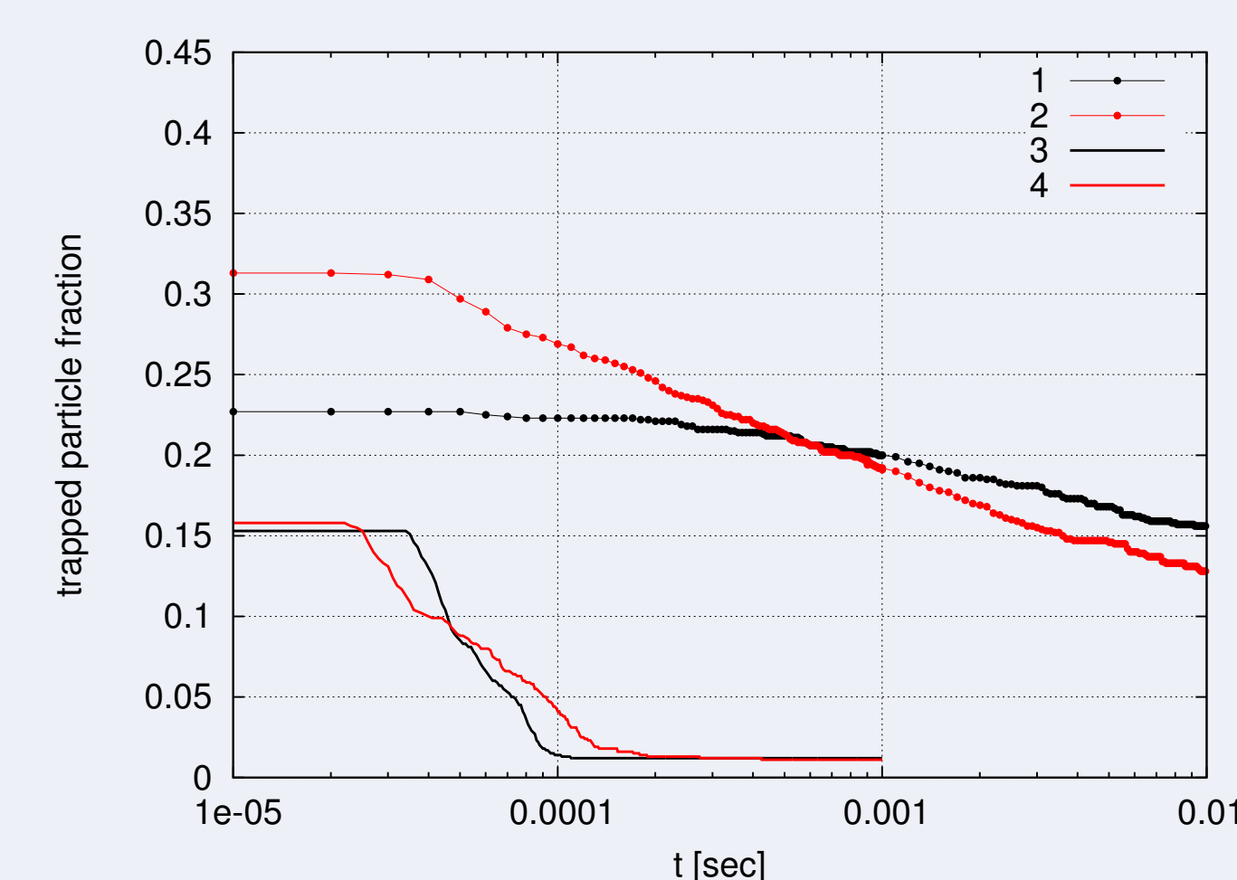
Fig. 3. Collisionless evolution of trapped \alpha -particle fraction for U-3M adapted to reactor parameters for inward shifted configurations (plots 1 and 2, with points) and standard configurations (plots 3 and 4, with lines). Particles are started on the magnetic surfaces corresponding to r/a \approx 0.25 (plots 1 and 3, black) and r/a \approx 0.5 (plots 2 and 4, red).
