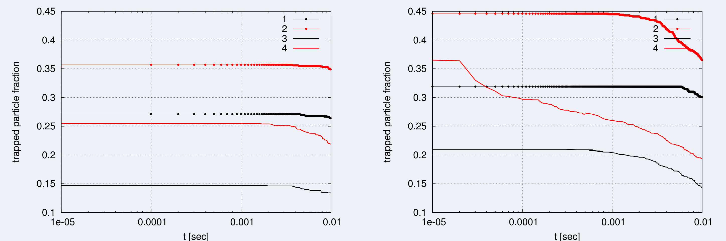
Fig. 2. Collisionless evolution of trapped \alpha -particle fraction for CHS (left) and LHD (right) adapted to reactor parameters for inward shifted configurations (plots 1 and 2, with points) and standard configurations (plots 3 and 4, with lines). Particles are started on the magnetic surfaces corresponding to r/a \approx 0.25 (plots 1 and 3, black) and r/a \approx 0.5 (plots 2 and 4, red).
