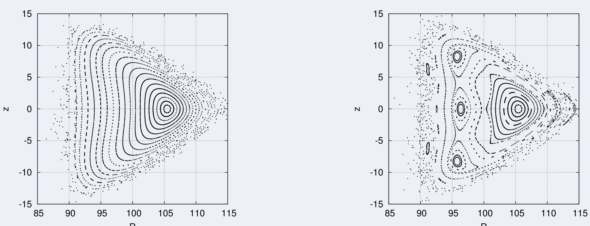
Fig. 1. Magnetic surfaces of the U-3M standard configuration without a small eccentricity in the vertical field coils (left) and with such eccentricity (right).
