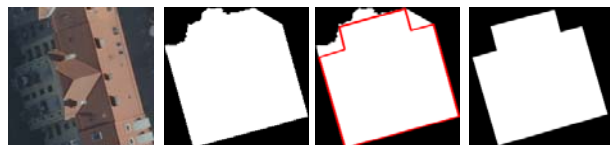
Figure 8: (a) building visible in vertical aerial image (b) segmentation result (c) in red modified building outline using 3D façade reconstruction (d) enhanced building footprint.
