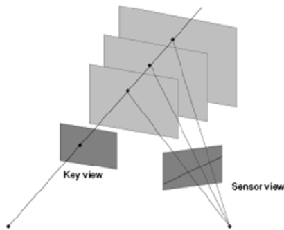
Figure 4: Plane sweeping principle. The homography between the façade's reference plane and the sensor view varies for different depths. (Zach, 2007).
