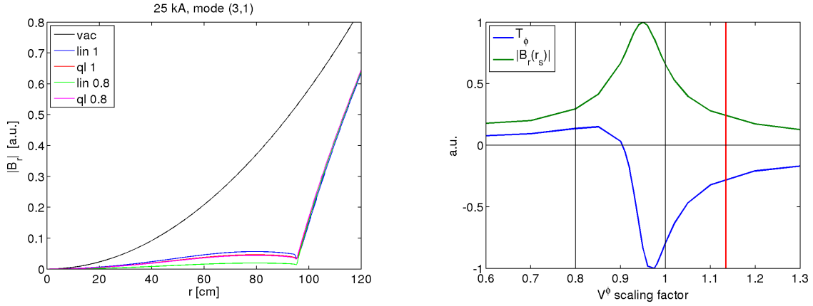
Fig. 1. Left: Radial profiles of |B_m^r| before and after quasilinear relaxation. Right: Toroidal torque and |B_m^r| at the resonant surface as functions of the toroidal velocity scaling factor. Starting scaling factor values used for the computations shown on the left (see legend) and the value corresponding to zero electron fluid velocity at the resonant surface are indicated by the black lines and the red line respectively on the right.
