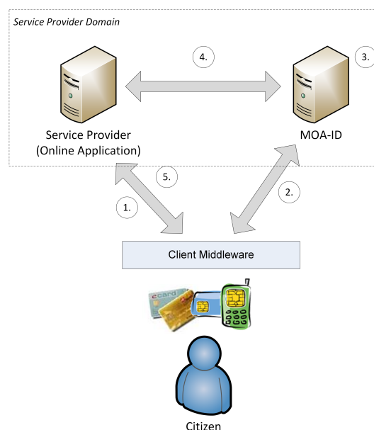
Figure 1: The basic Austrian eID system Architecture
