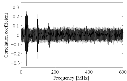
Fig. 5. Result of the DFA attack on the HF-tag prototype.
