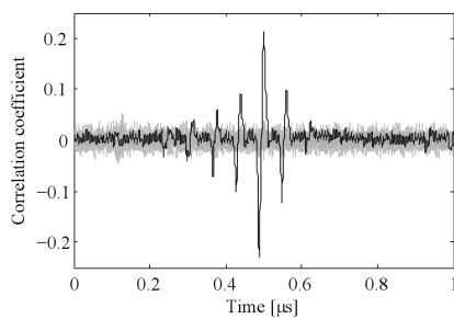
Fig. 8. Result of the windowing attack on the HF-tag prototype.
