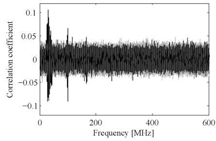
Fig. 9. Result of the DFA attack on the HF-tag prototype.
