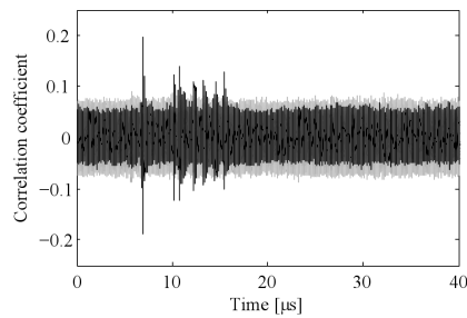
Fig. 4. Result of the filtered DEMA attack on the HF-tag prototype.
