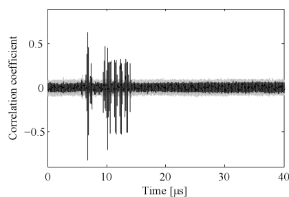
Fig. 6. Result of the filtered DEMA attack on the UHF-tag prototype.
