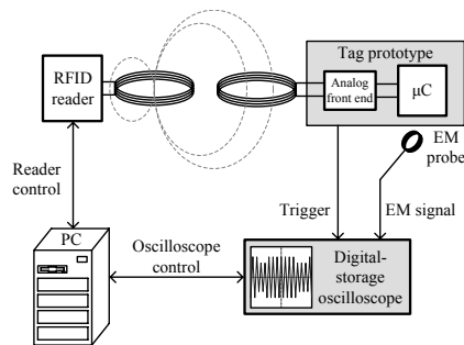
Fig. 2. Schematic view of the general measurement setup.
