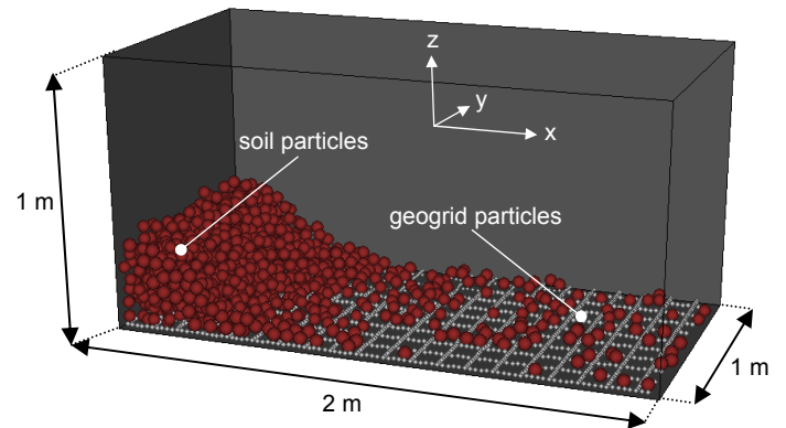
Figure 2. Generated model with the Particle Flow Code.
