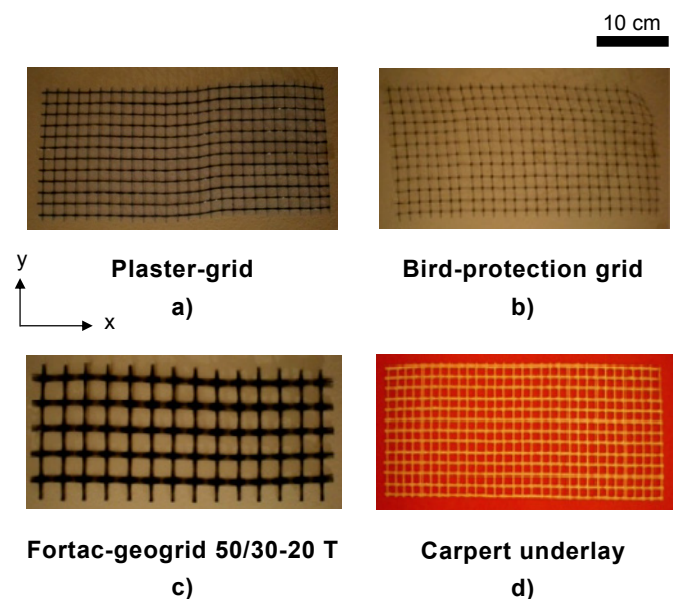
Figure 4. Soft material validation for small scale labtest.
