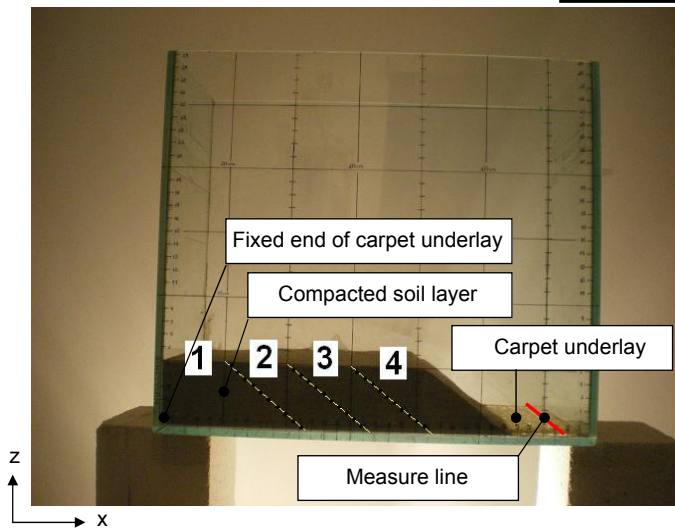
Figure 5. Frontview of the small scale prestressing test during filling and compaction process
