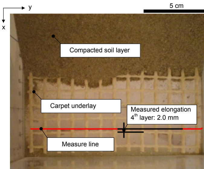
Figure 6. Topview of the small scale prestressing test after filling and compaction to measure the grids elongation
