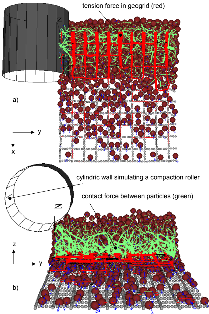
Figure 3. Discrete model of granular soil, geogrid and compaction roller (the thickness of the red lines represents the tensile force in the geogrid string. a) Topview b) Frontview
