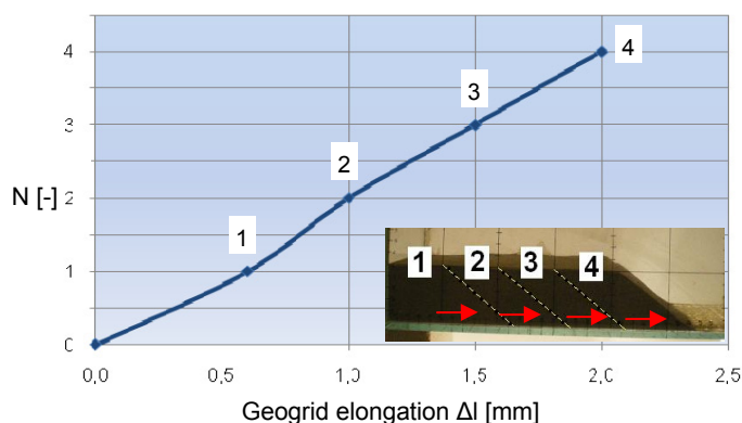
Figure 7. Geogrids elongation after filling and compacting with the compaction advice (Chapter 2)
