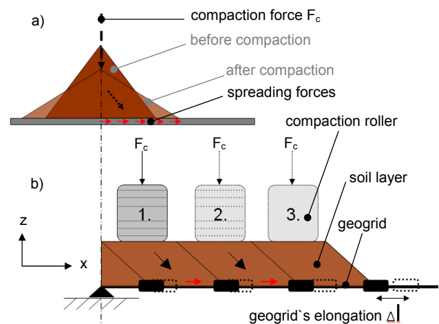
Figure 1. a) Principle to constitute spreading stresses during compaction b) Compaction advice to prestress the geogrid
