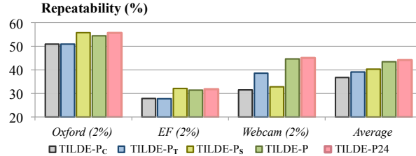
Figure 6: Effects of the three terms of the objective function, and of the approximation using separable filters.
