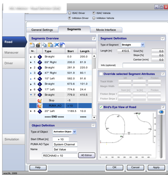
Figure 3: Screenshot of the lo-fi prototype.
