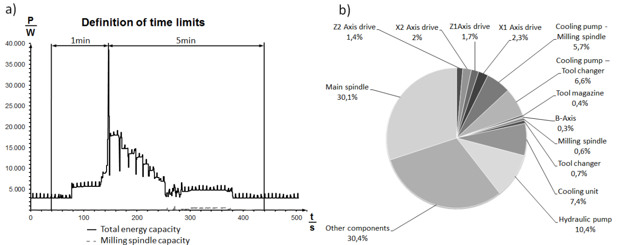
Figure 2: a) Total power consumption of the CNC lathe b) Energy distribution when manufacturing a test workpiece
