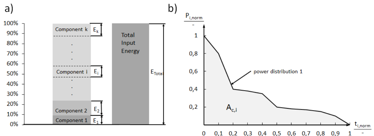
Figure 1: Example of an energy distribution of a machine tool.
