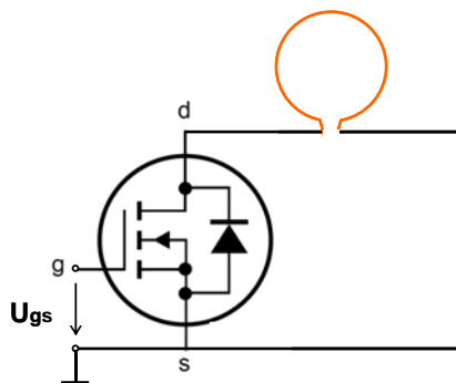
Figure 1. Active marker consisting of a wire loop and a CMOS switch for shorting the loop.
