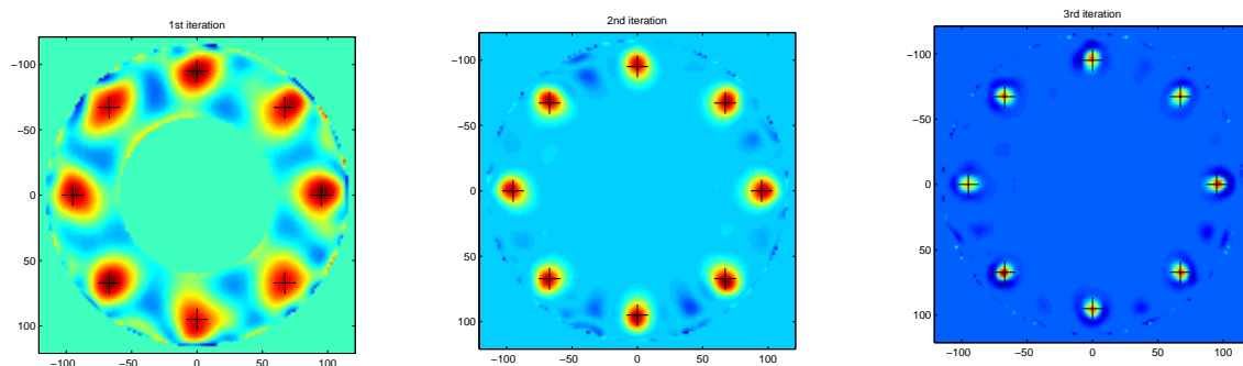
Figure 3. Reconstructed position of the markers after one, two and three iterations. The crosses mark the true positions
