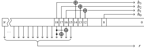
Figure 3: The reverse-engineered DRAM addressing functions from our Chromebooks.
