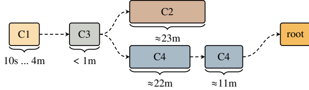
Figure 8: The timing durations for the end-to-end exploit executed on the Chromebook 2 . For Challenges C1 and C4 faster alternatives might be available (cf. Sections 6.1 and 6.4). The overall runtime is bound by Challenge C2 , i.e. , the time it takes to induce an exploitable bit flip. Afterwards it takes on average halve C4 to find the bit flip.
