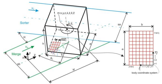
Fig. 8. 2D - MBD-Model
