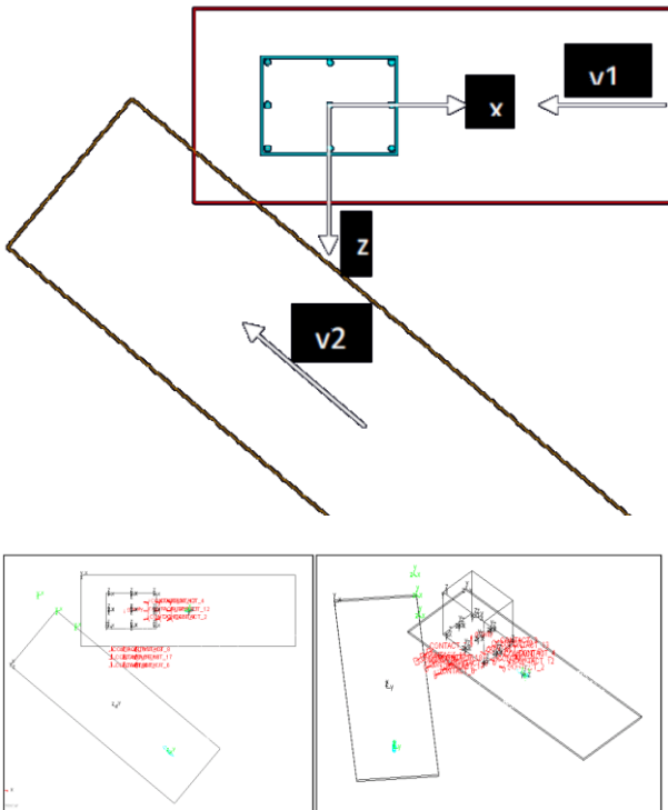
Fig. 7. in-feed with the conveyor- model from 3.1, and the conveyor-piece good contact from 4.1 with characteristic points of contact, represented in CAD-geometry
