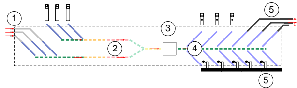
Fig. 3. Sortation system [1, 6].
