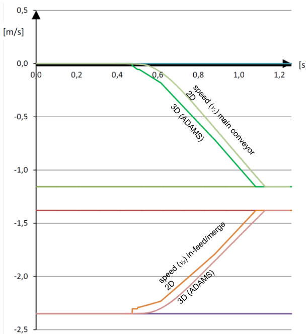
Fig. 9. in-feed with the 2D and 3D in-feed model. Friction forces and speeds in x and z direction.
