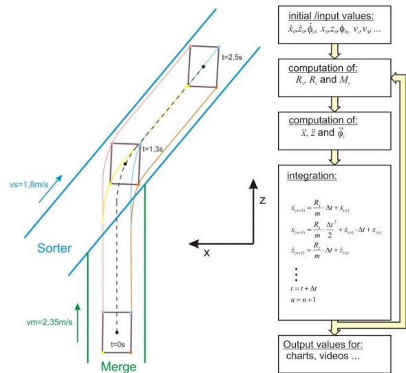
Fig. 10. Flow diagram and trace curves of the feed-in process
