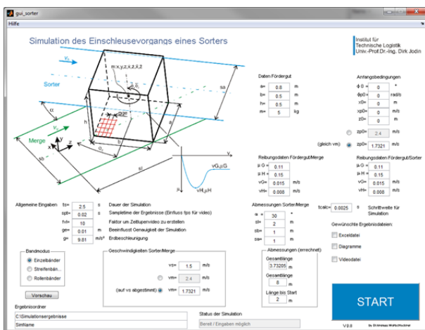
Fig. 9. GUI of the 2D-approach for the in-feed
