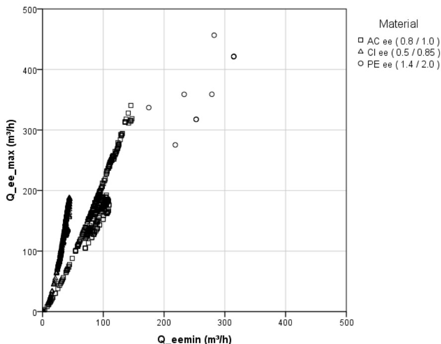
Figure 1: Comparison of leakage outflow for longitudinal cracks (width=2mm; length = 1m; A = 20cm 2 ) and different emitter exponents ( e_e ) in a partial transmission mains system of Vienna
